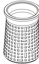
CONCRETE: WS101 26" D X 36" H, 850 LBS. 31-GALLON LINER
